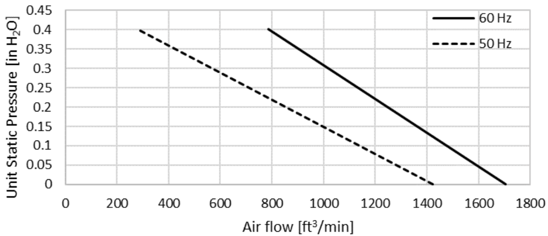
Fan at Low Speed (imperial units)
