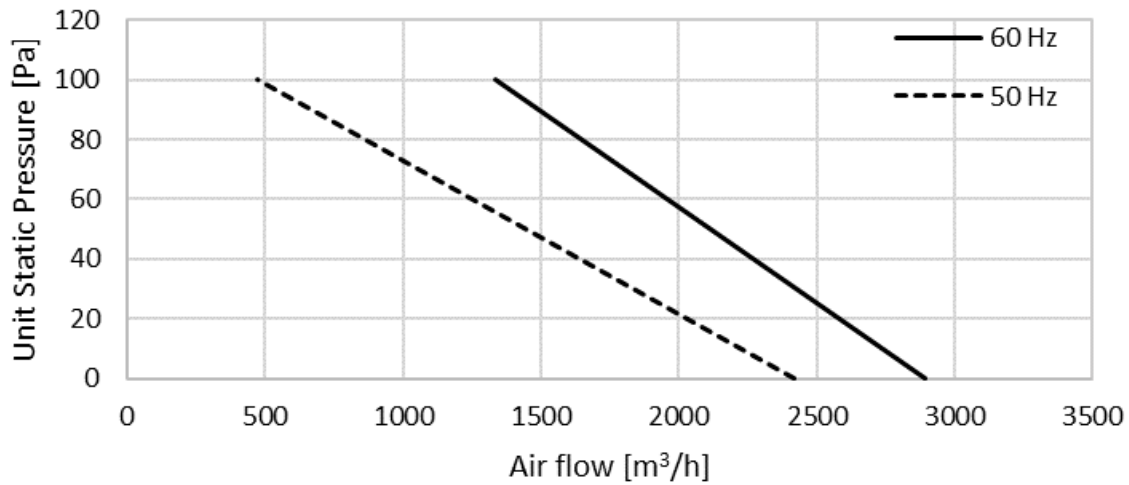
Fan at Low Speed (metric units)
