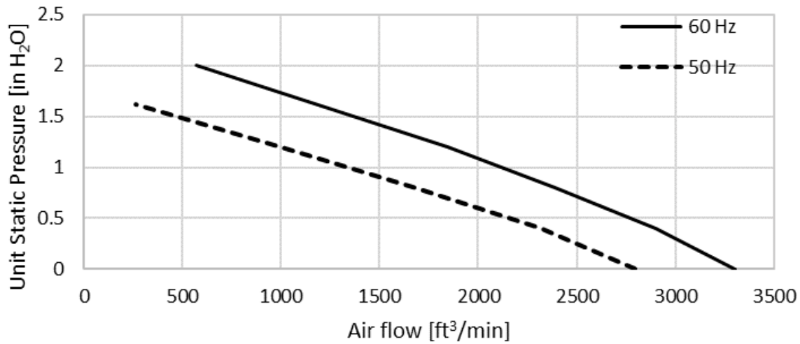
Fan at High Speed (imperial units)
