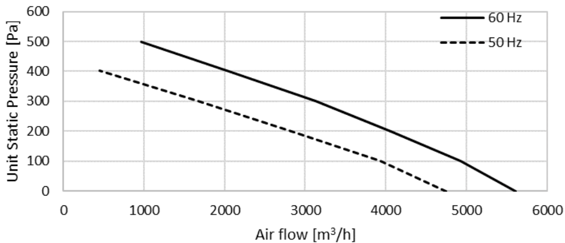
Fan at High Speed (metric units)
